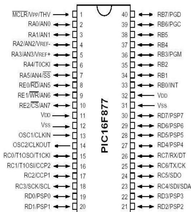
Fig 4 PIC controller
