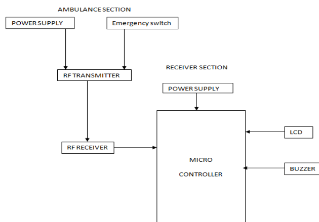
Fig.2. RF Transmitter and Receiver
