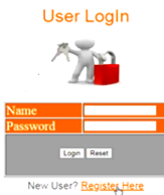
Figure 3 User Login
