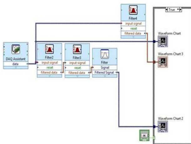
Fig 8: The integration processing of EMG signals.
