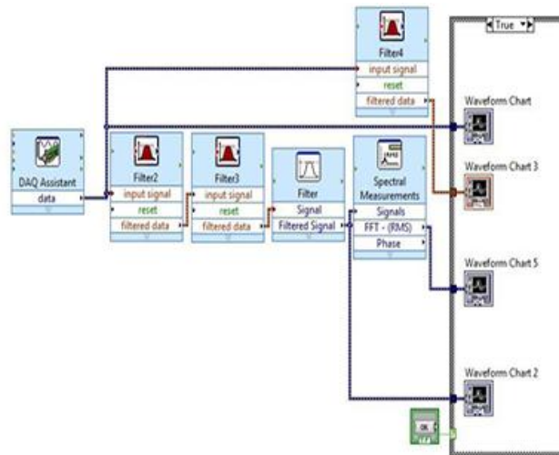
Fig 8: The RMS processing of EMG signals.
