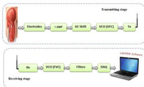
Fig 1: Block diagram of the proposed overall Wireless Electromyography (EMG) system design.
