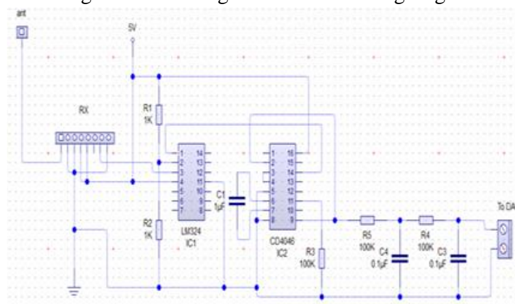
Fig4: Circuit Diagram of Receiving stage.
